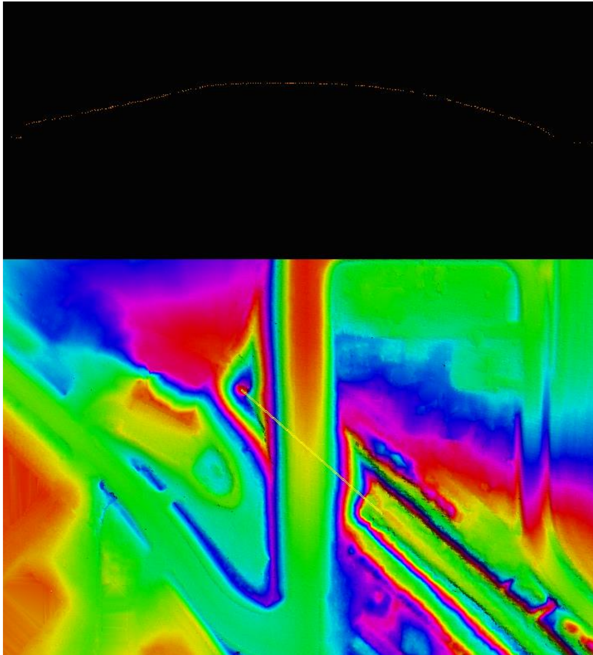
Figure 23: Profile with points colored by class (class 1=white, class 2=orange) is shown in the top view and the DEM is shown in the bottom view. This culvert remains in the bare earth surface. Bridges have been removed from the bare earth surface and classified to class 17.
