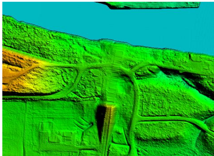
Figure 22: DEM with bridge removed from surface model.
