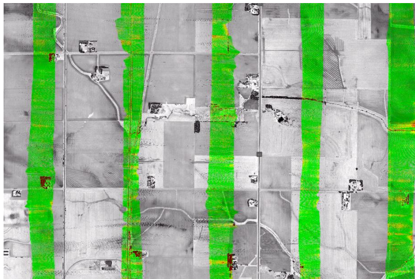
Figure 17: DZ Ortho of inter-swath
