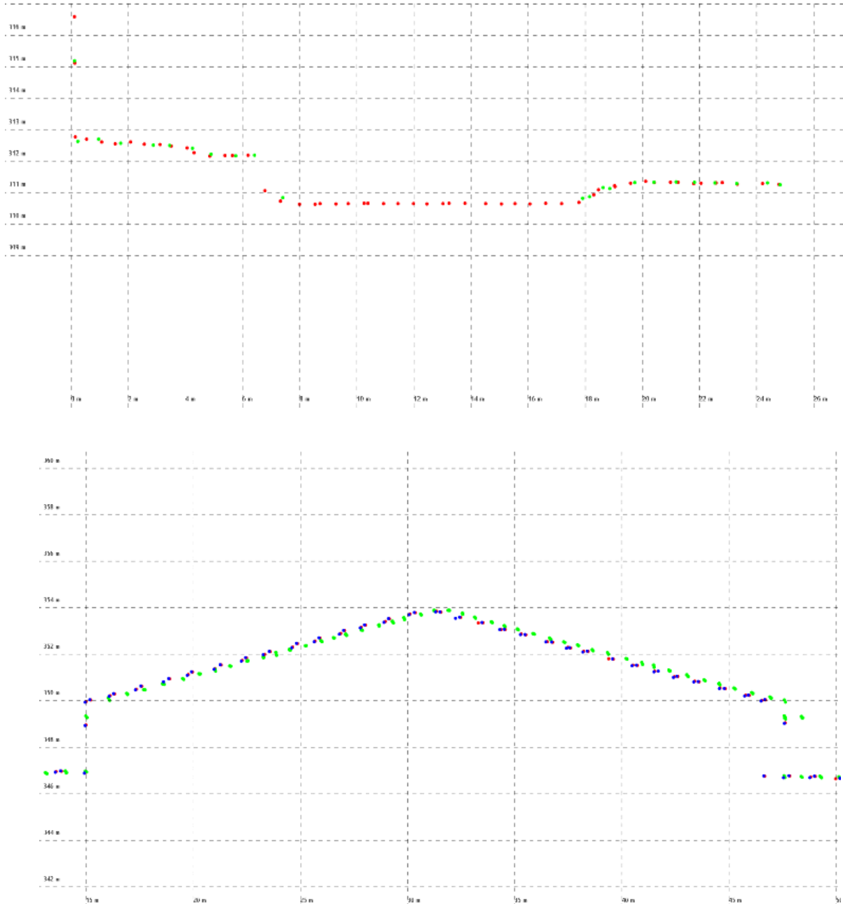
Figure 13: Profile views showing correct roll and pitch adjustments
