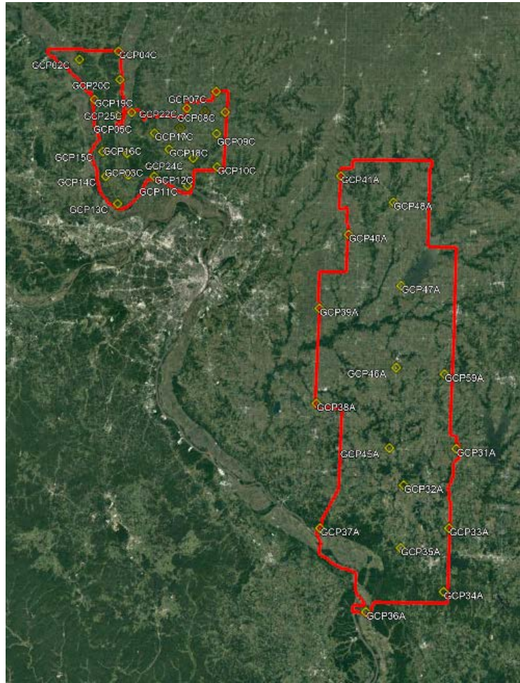
Figure 13: surveyed Ground Control Point Locations
