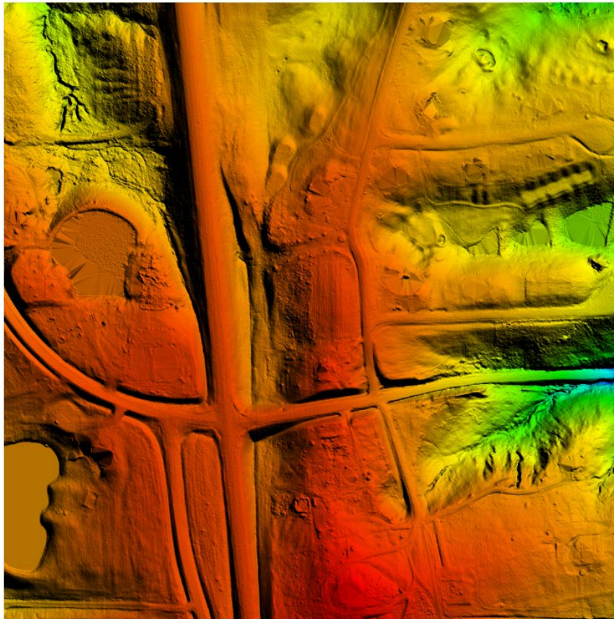
Figure 26: IL South Central project bare earth DEM
