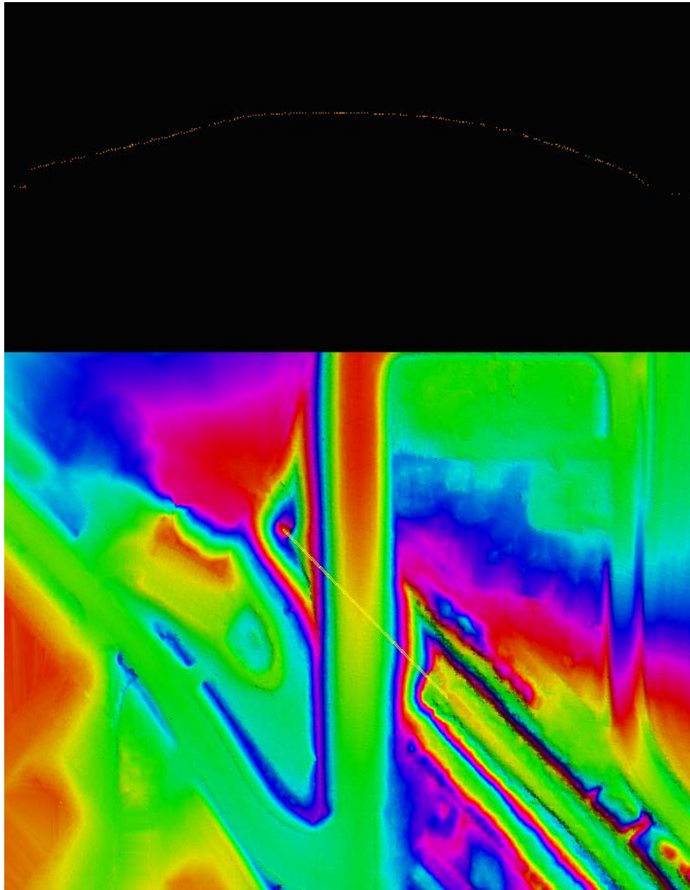
Figure 19: Profile with points colored by class (class 1=white, class 2=orange) is shown in the top view and the DEM is shown in the bottom view. This culvert remains in the bare earth surface. Bridges have been removed from the bare earth surface and classified to class 17.
