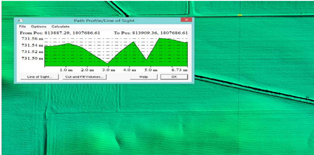
Figure 21: The flight line ridge is less than 8 cm. Overall; the IL South Central project data meets the project specifications for 8 cm RMSDz relative accuracy requirement
