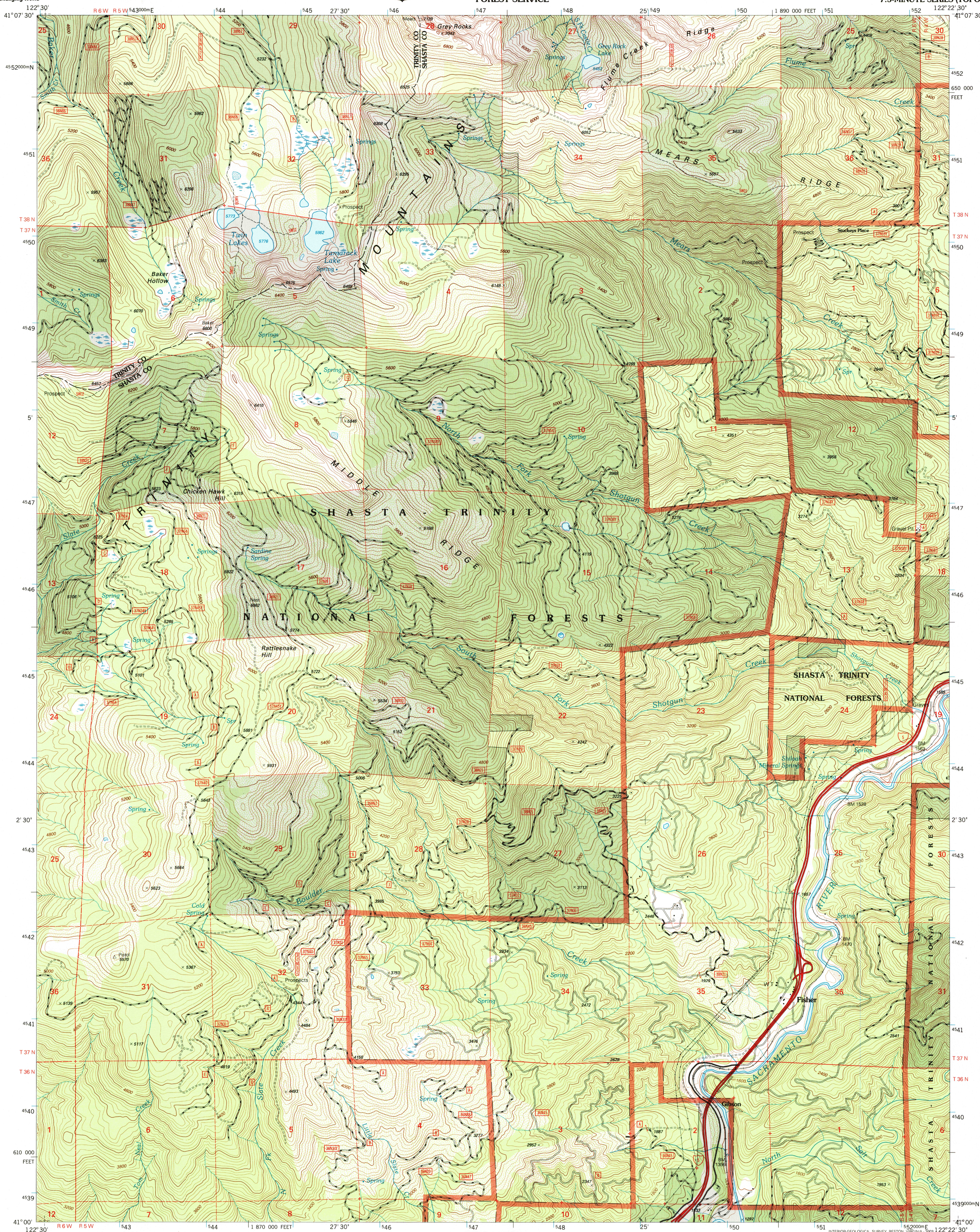
QUADRANGLE LOCATION
