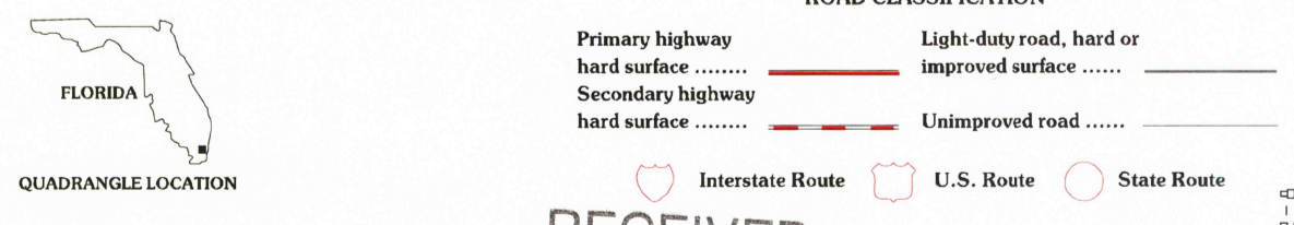
QUADRANGLE LOCATION
